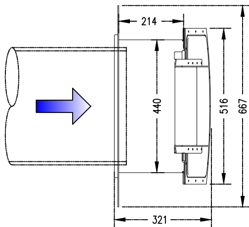
① TOP VIEW
