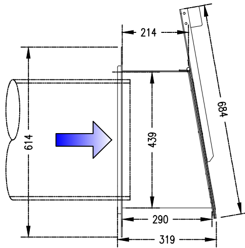
② SIDE VIEW
